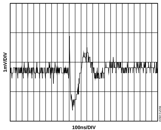
Figure 26. DAC-to-DAC Crosstalk
